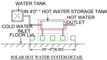
SOLAR HOT WATER SYSTEM DETAIL
