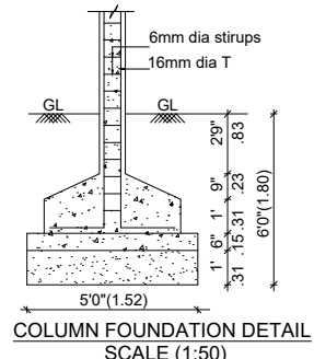
COLUMN FOUNDATION DETAIL SCALE (1:50)
