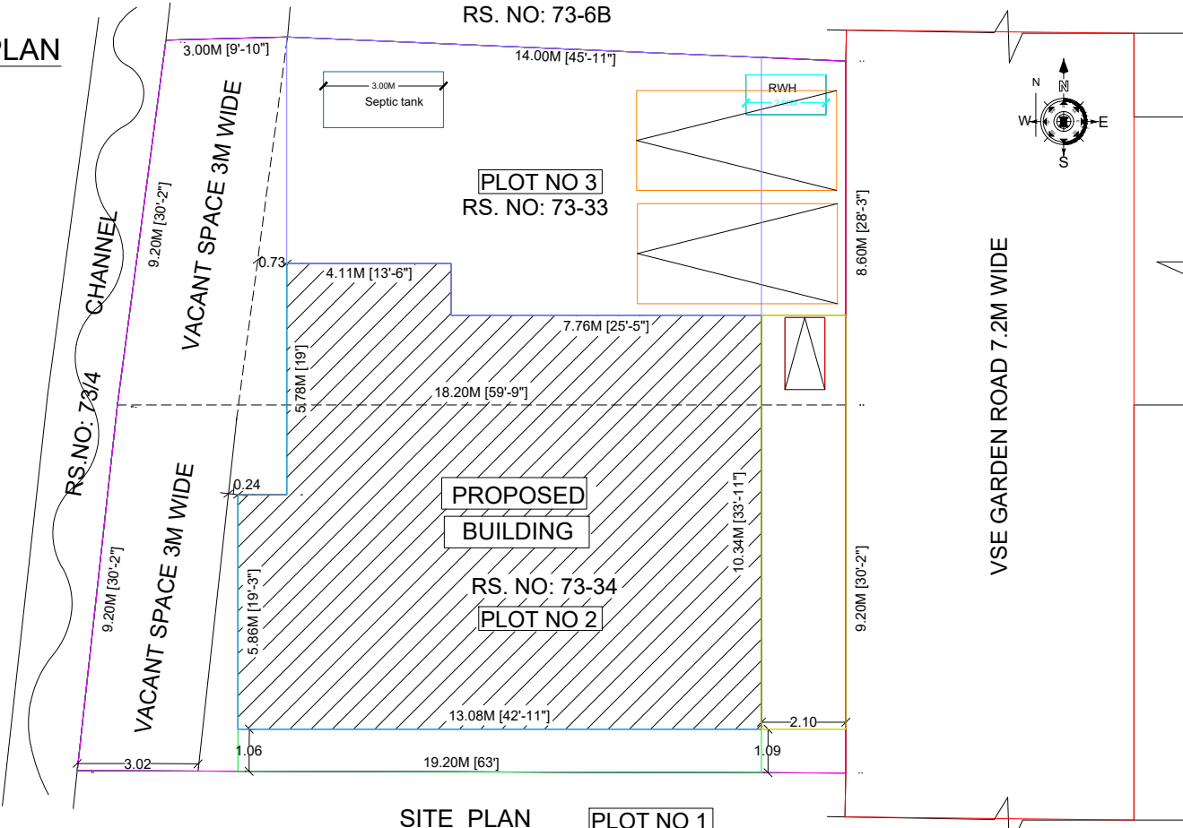
SITE PLAN
