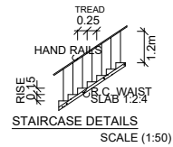
STAIRCASE DETAILS SCALE (1:50)
