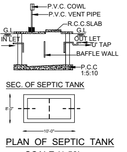
PLAN OF SEPTIC TANK SCALE (1:50)
