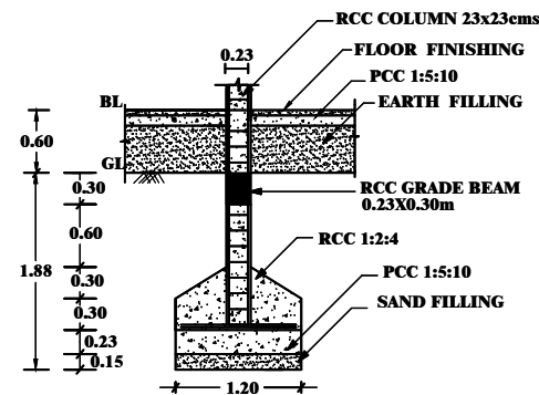
FOUNDATION DETAILS
