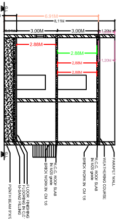
SECTION ON XX
