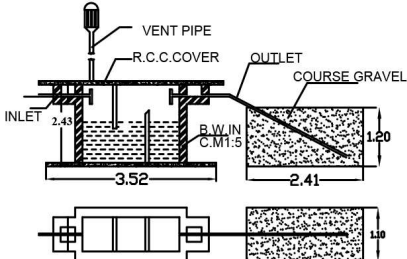
SEPTIC TANK & D-TRENCH DETAILS
