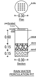
RAIN WATER PERCOLATION PIT
