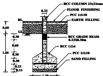
FOUNDATION DETAILS
