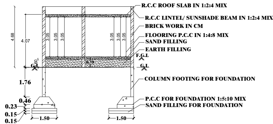
SECTION ON-SD
