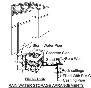
RAIN WATER STORAGE ARRANGEMENTS
