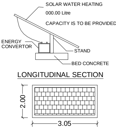
SOLAR SYSTEM
