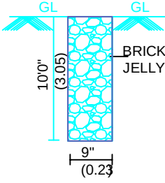
PERCOLATION PIT
