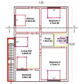
PROPOSED GROUND FLOOR PLAN
