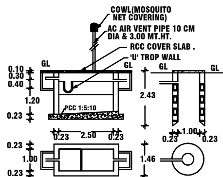
PLAN AND CROSS SECTION OF ST&SP.
