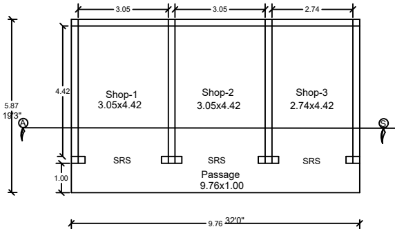
PROPOSED. G.F. PLAN.
