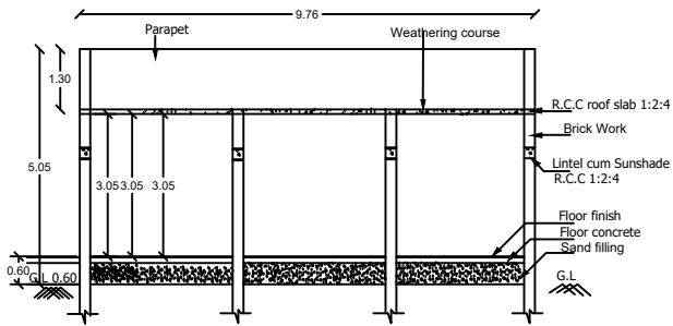
SECTION ON "A S"
