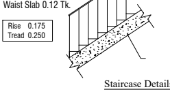
Staircase Details
