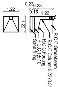
Foundation details-2
