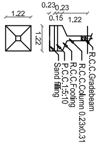
Foundation details-1
