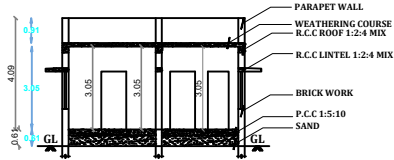
SECTION ON - "SP"
