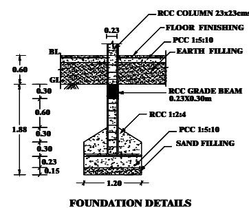
FOUNDATION DETAILS
