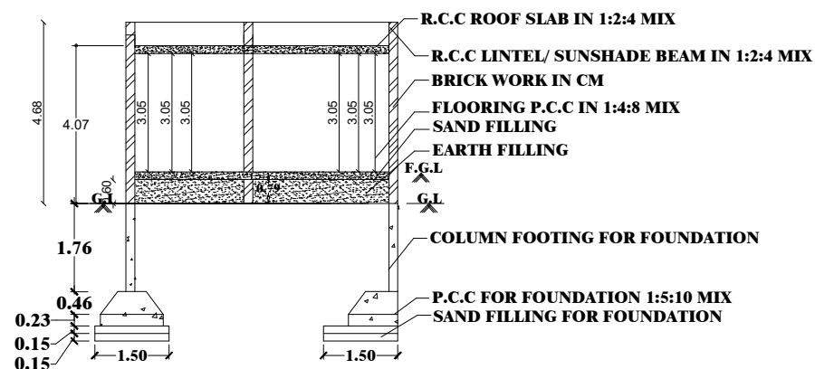
SECTION ON-SD
