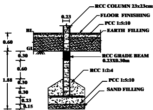
FOUNDATION DETAILS
