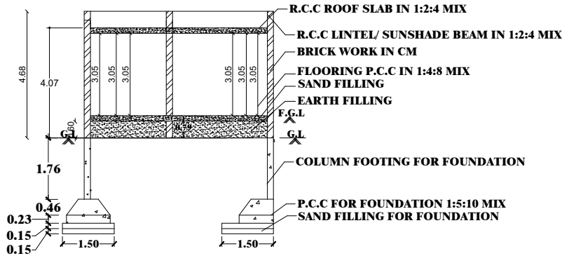
SECTION ON-SD
