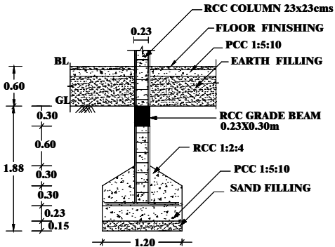
FOUNDATION DETAILS
