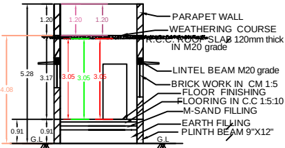
SECTION ON XX
