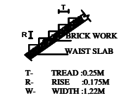
STAIRCASE DETAILS (NOT TO SCALE)
