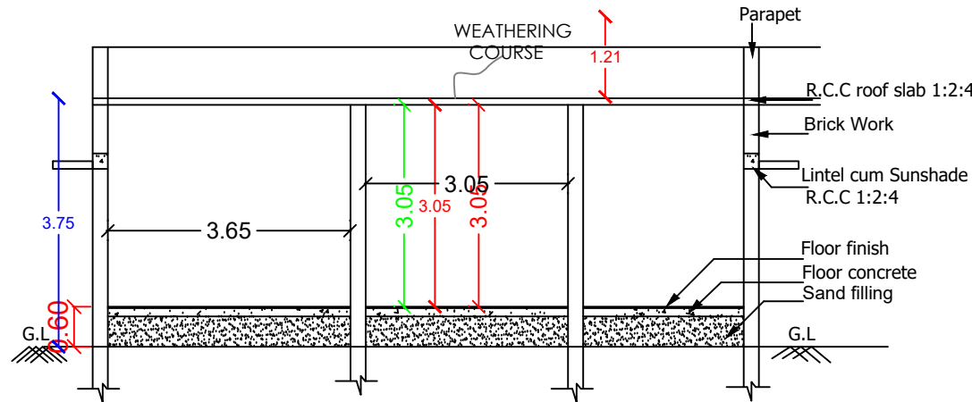
SECTION ON "A S"
