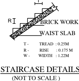
STAIRCASE DETAILS (NOT TO SCALE)
