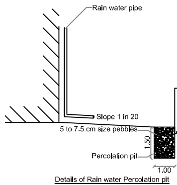
Details of Rain water Percolation pit
