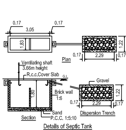
Details of Septic Tank
