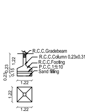
Foundation details
