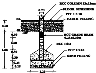
FOUNDATION DETAILS
