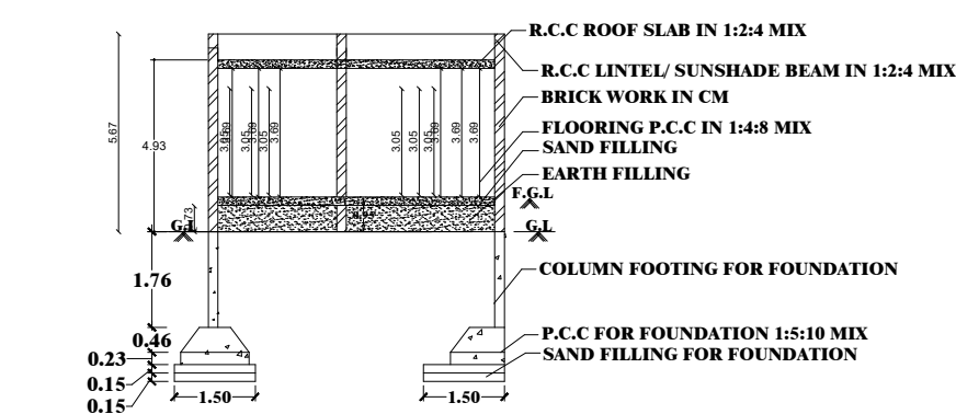
SECTION ON-SD
