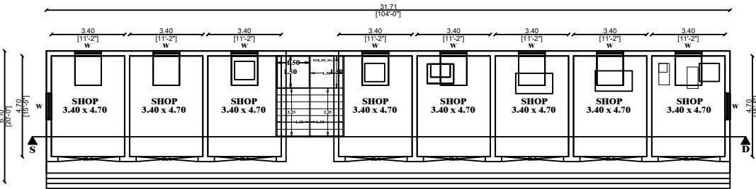
PROPOSED GROUND FLOOR PLAN
