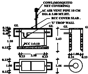
PLAN AND CROSS SECTION OF ST&SP.
