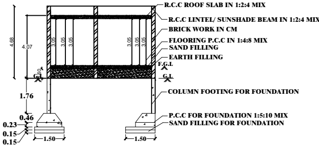
SECTION ON-SD
