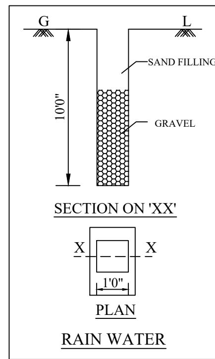
RAINWATER HARVESTING
