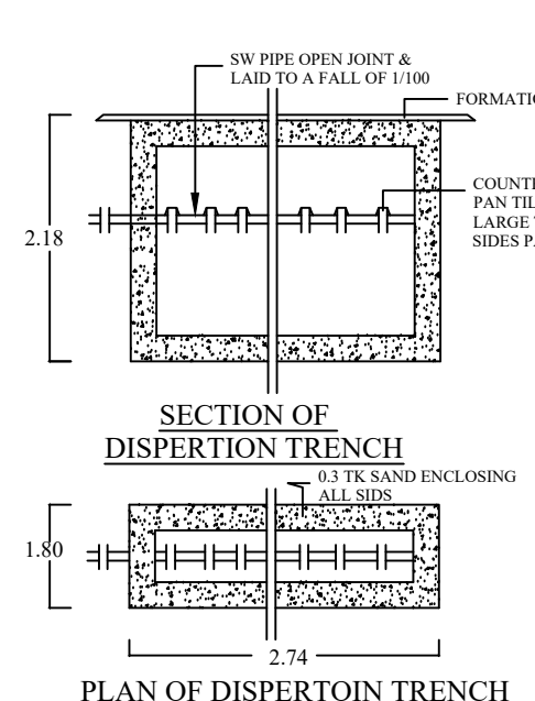
DISPERSION TRENCH
