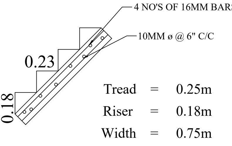
STAIRCASE DETAILS
