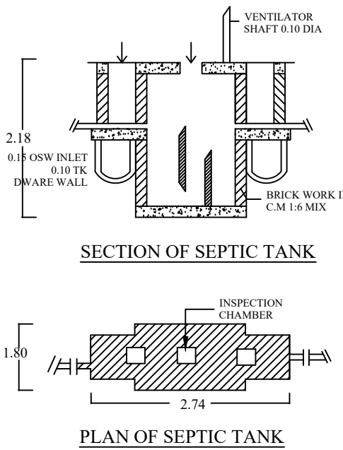
SEPTIC TANK
