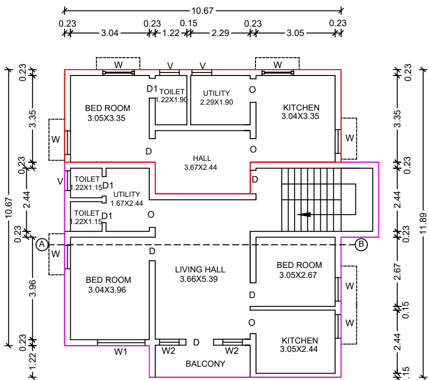
PROPOSED ADDITIONAL CONSTRUCTION OF FIRST FLOOR PLAN
