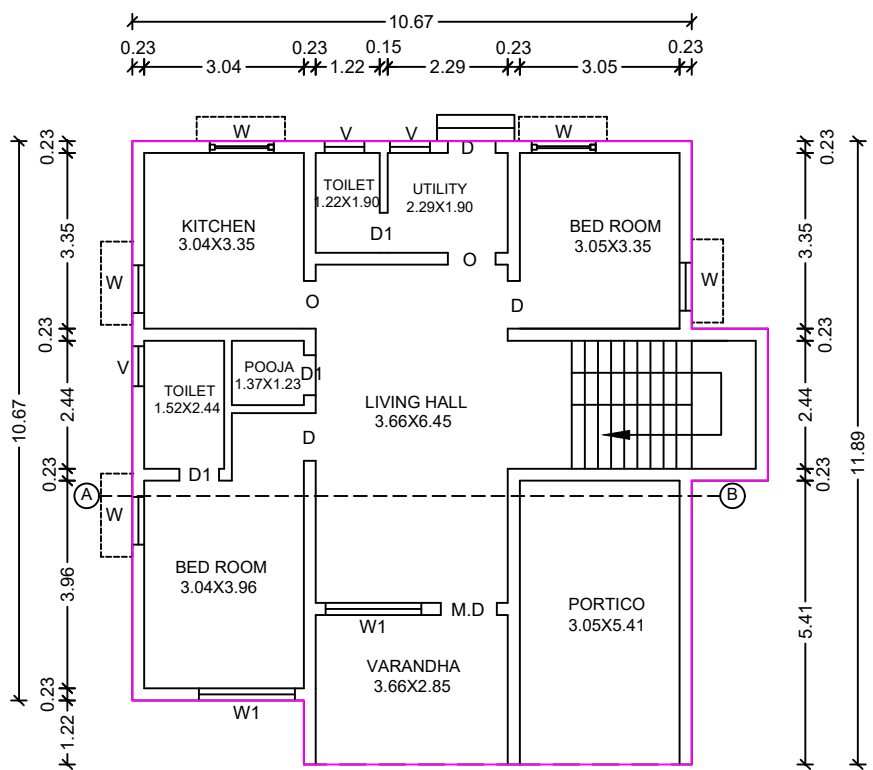
EXISTING APPROVED GROUND FLOOR PLAN
