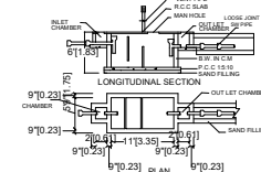
SEPTIC TANK
