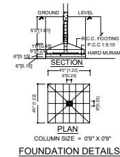
FOUNDATION DETAILS
