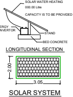
SOLAR SYSTEM
