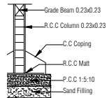
Percolation Detail
