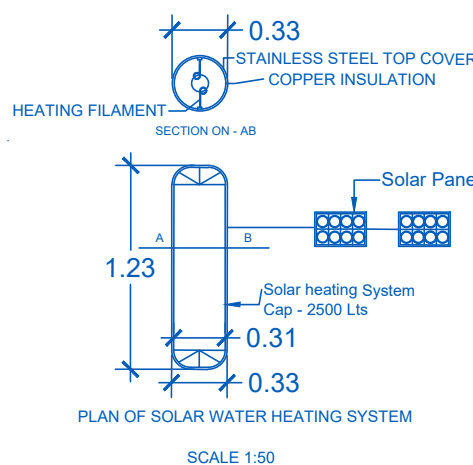
SCALE 1:50
