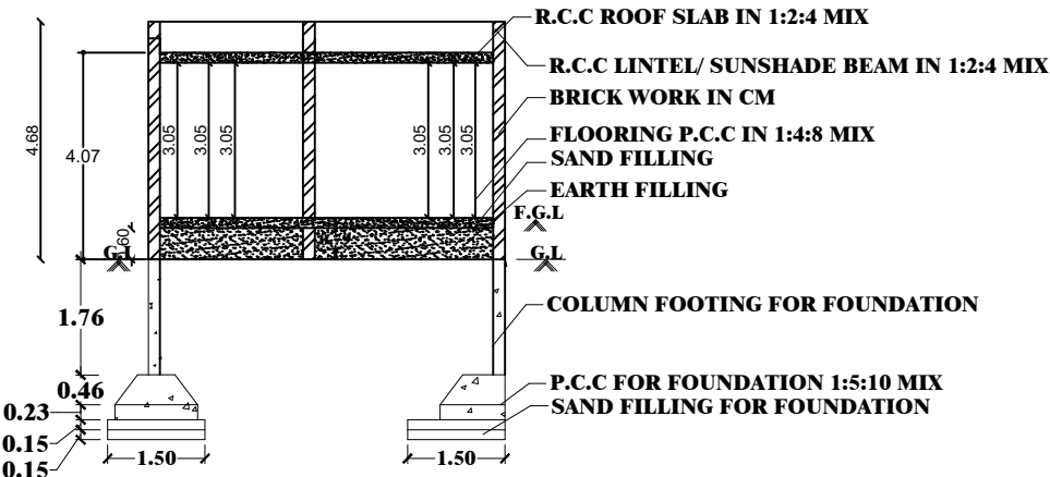
SECTION ON-SD
