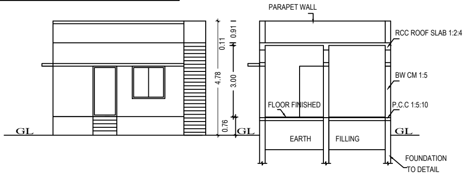
FRONT ELEVATION
