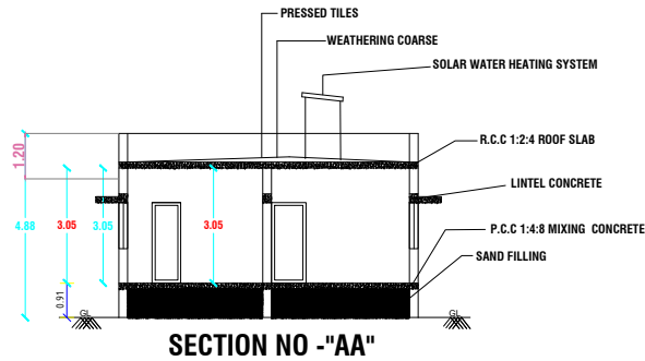
SECTION NO -"AA"
