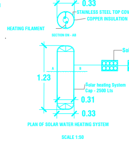
PLAN OF SOLAR WATER HEATING SYSTEM SCALE 1:50
