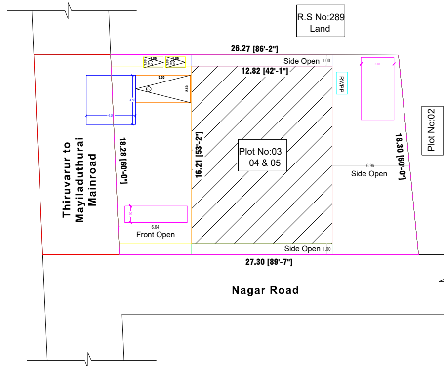
N ↑ SITE PLAN
