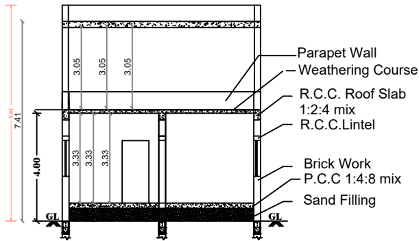
SECTION ON - SD
