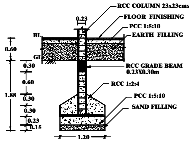
FOUNDATION DETAILS
