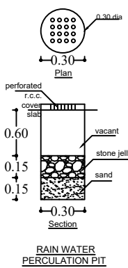
RAINWATER PERCOLATION PIT
