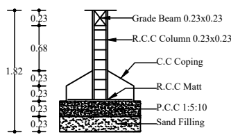
Foundation Detail
