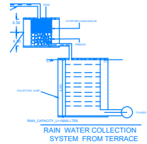
RAIN WATER COLLECTION SYSTEM FROM TERRACE
