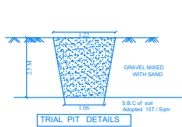
TRIAL PIT DETAILS
