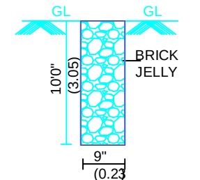
PERCOLATION PIT
