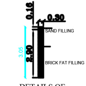
DETAILS OF PERCULATION PIT RWHL_CAPACITY_L=1000 LTRS
