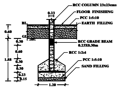
FOUNDATION DETAILS
