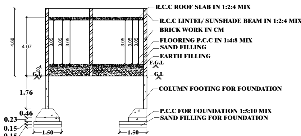
SECTION ON-SD
