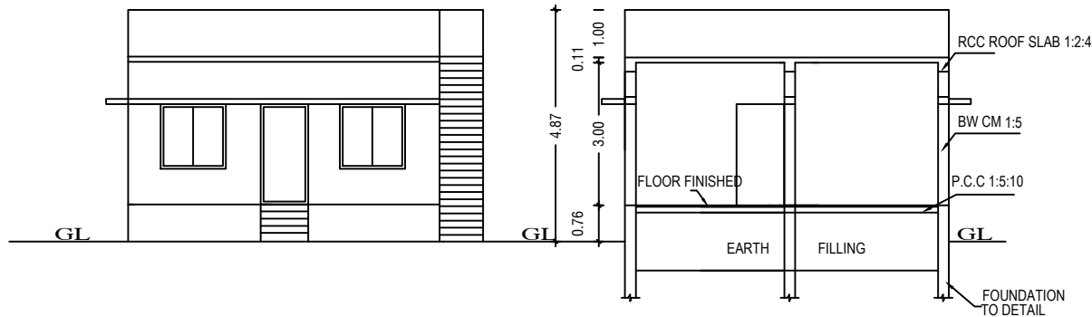
FRONT ELEVATION
