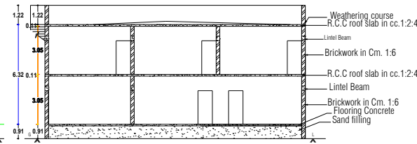
SECTION ON 'AB'
