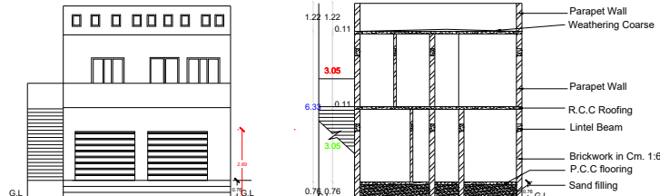
FRONT ELEVATION
