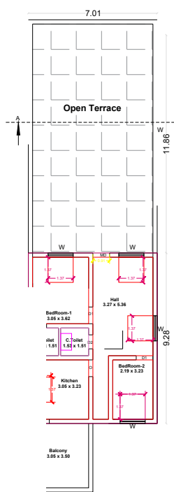
FIRST FLOOR PLAN (Residential Building)
