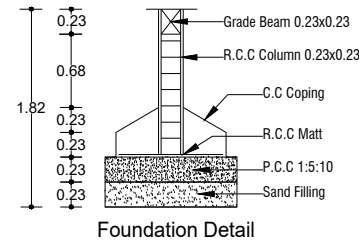
Foundation Detail
