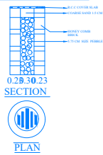
PLAN
