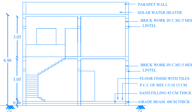
SECTION- AA1
