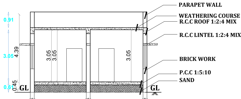
SECTION ON - "SP"
