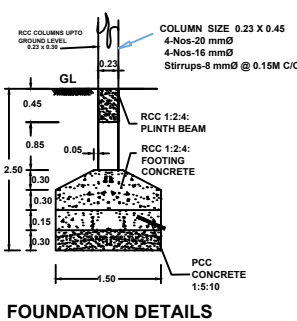
FOUNDATION DETAILS
