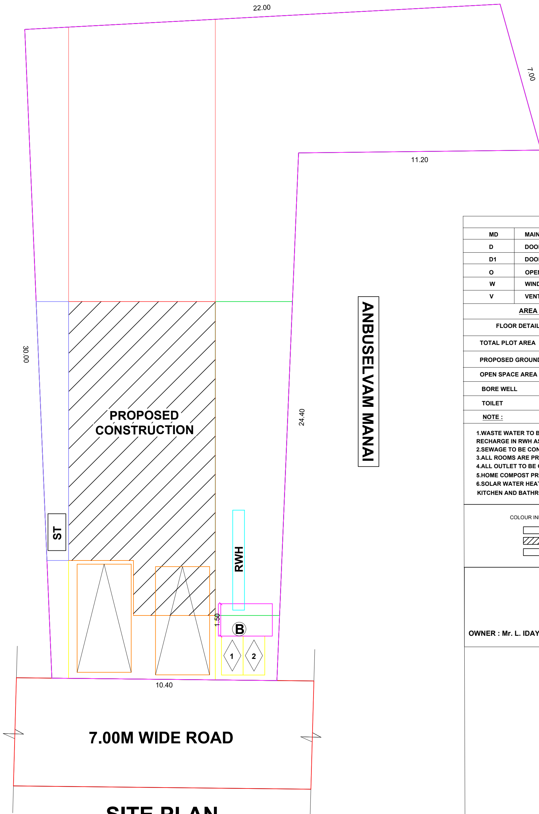
SITE PLAN
