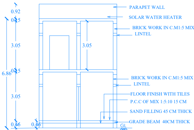
SECTION- AA1
