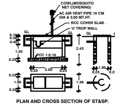
PLAN AND CROSS SECTION OF STEP
