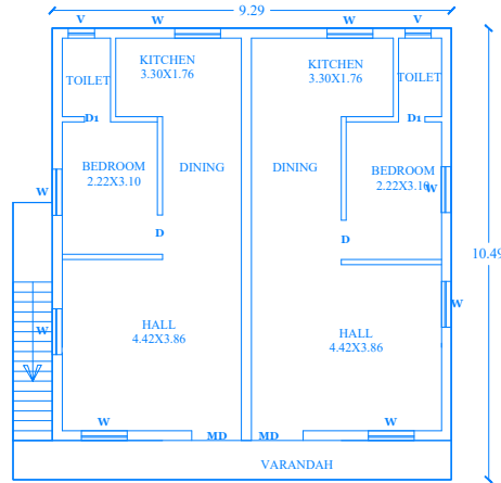
EXI-FIRST FLOOR & ADD FIRST FLOOR PLAN
