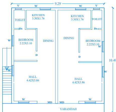
EXI-GROUND FLOOR & ADD GROUND FLOOR PLAN
