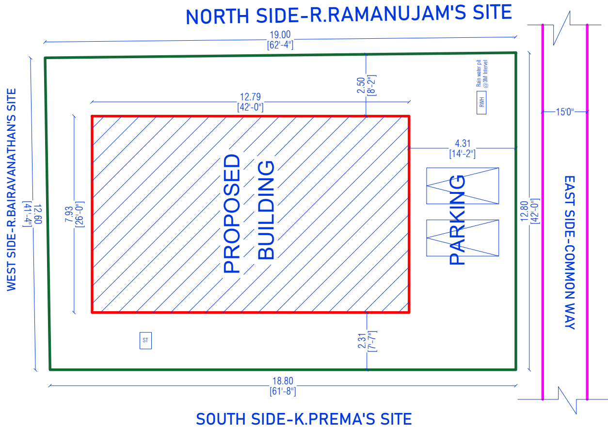
SITE PLAN
