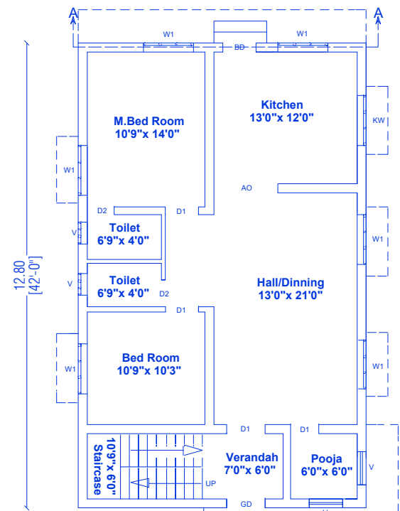
PRO-GROUND FLOOR
