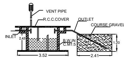
SEPTIC TANK & D-TRENCH DETAILS
