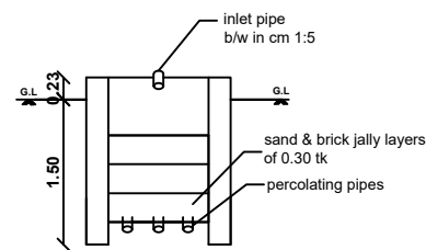
SECTION OF RAIN WATER HARVESTING PIT
