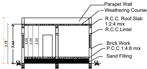
SECTION ON - SD
