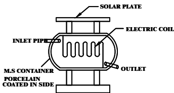
SOLAR SYSTEM
